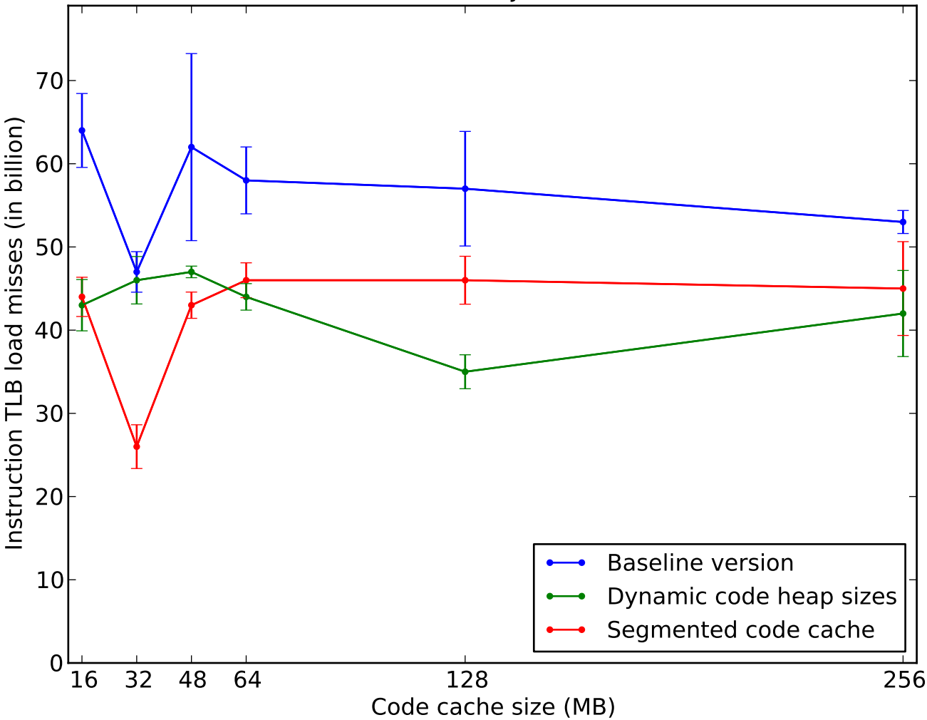
Instruction TLB behaviour (SPECjbb2005 Benchmark, 32-core)
