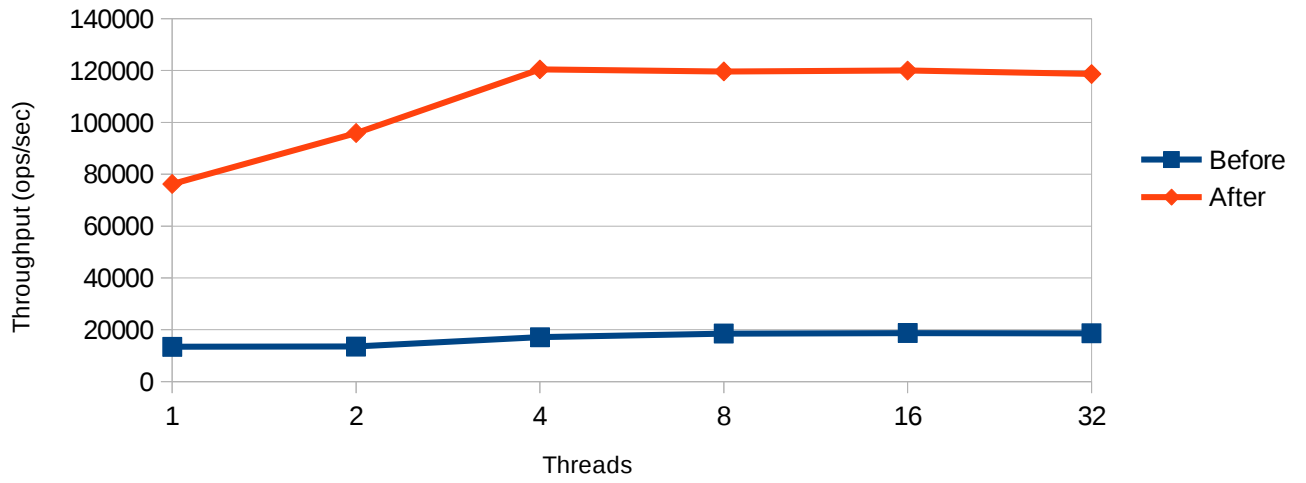
SecurityManager.checkPackageAccess(String)
